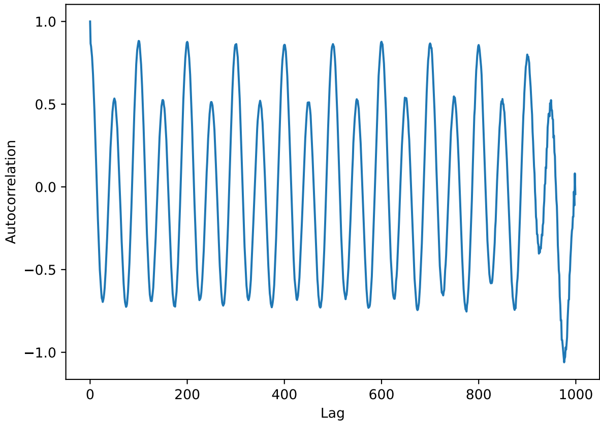
Autocorrelation of y
